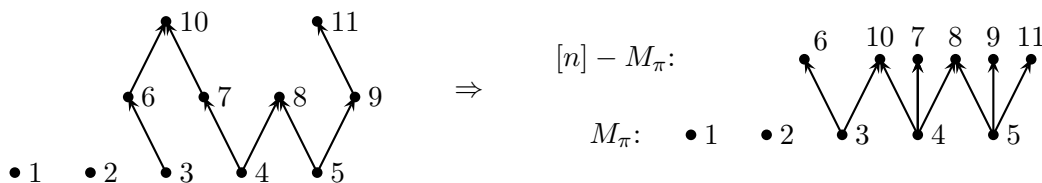
Figure 2: Example of a dag (left) and its associated bipartite partial order (right).
