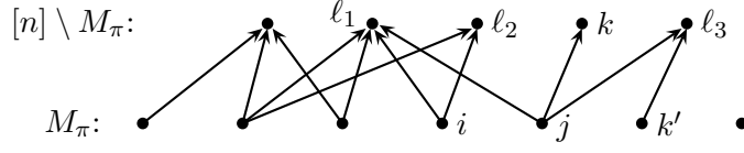
Figure 3: A bipartite partial order \pi is pictured, with the ordered pairs of \pi shown as directed edges. (For instance, j \prec_\pi k holds.) The set M_\pi is the set of minimal vertices. The nodes i, j, k shown are an example of nodes used for a transitivity axiom \bar{x}_{i,j} \vee \bar{x}_{j,k} \vee \bar{x}_{k,i} of type (\gamma) . The nodes i, j, k' are an example of the nodes for a transitivity axiom of type (\beta) .
