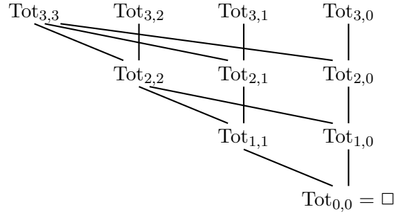
Figure 1: Main structure of the regular refutation P_n of the GT_n clauses, with n = 4 . Inferences that resolve against transitivity clauses T_{i,j,k} are not shown: the slanted line from Tot_{k+1,k+1} to Tot_{k,\ell} represents k many resolution inferences against the clauses T_{\ell,i,k+1} for i \in [k+1] \setminus \{\ell\} . Each subderivation with hypotheses Tot_{k,k} and Tot_{k,\ell} and conclusion Tot_{k-1,\ell} is an input derivation.
