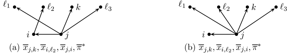
Figure 5: The partial orders for the fragment of S_2 shown in (7).
