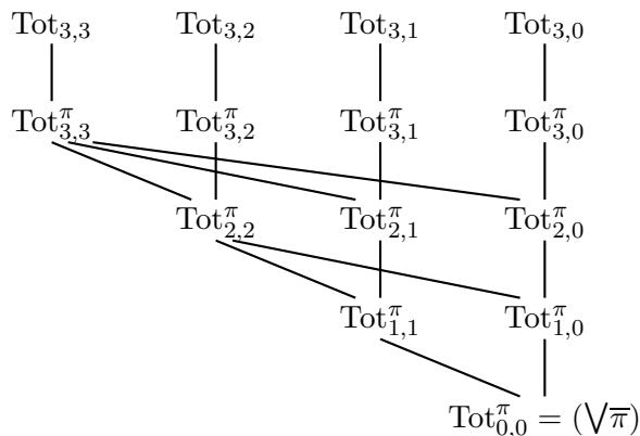
Figure 4: Main structure of the regular derivation P_\pi , with m = 4 . The initial clauses are \text{GT}_m clauses. Inferences that resolve against transitivity clauses T_{i,j,k} are not shown: slanted lines and the top row of vertical lines represent multiple resolution inferences against transitivity clauses.
